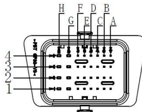
0643340100 Charger Low Voltage Connector
