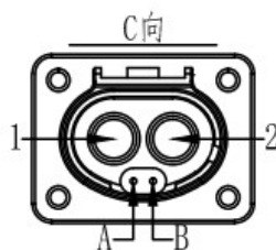
PL082X-61-10 OBC Output and DC-DC Input
