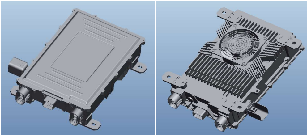
Chart 1 Fan-cooled Appearance
